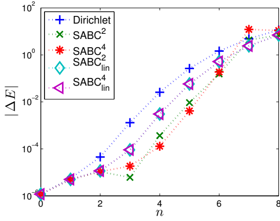
(a) x_r = 2 (loop)
