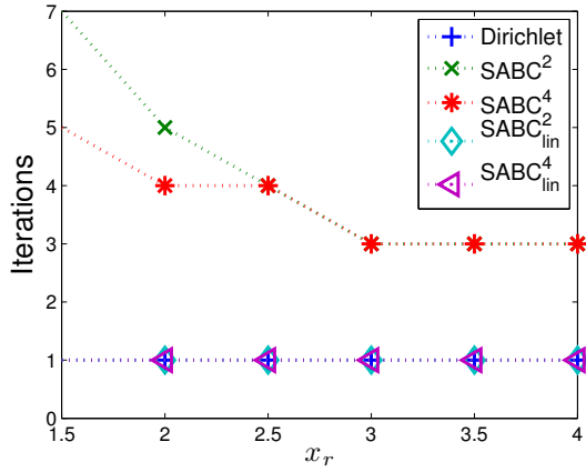
(a) n = 0
