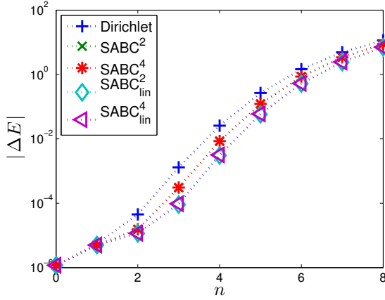
(c) x_r = 2 (direct)
