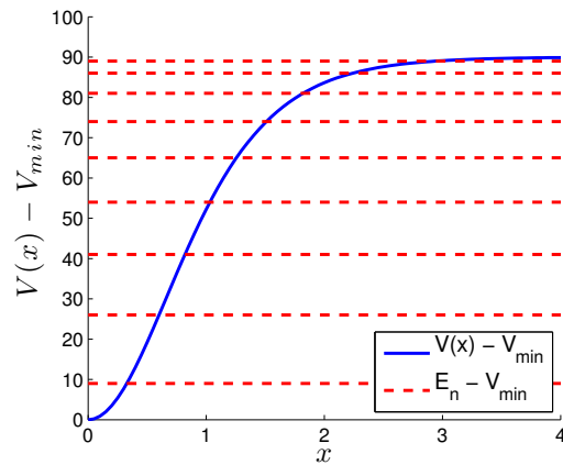
(b) Energy levels
