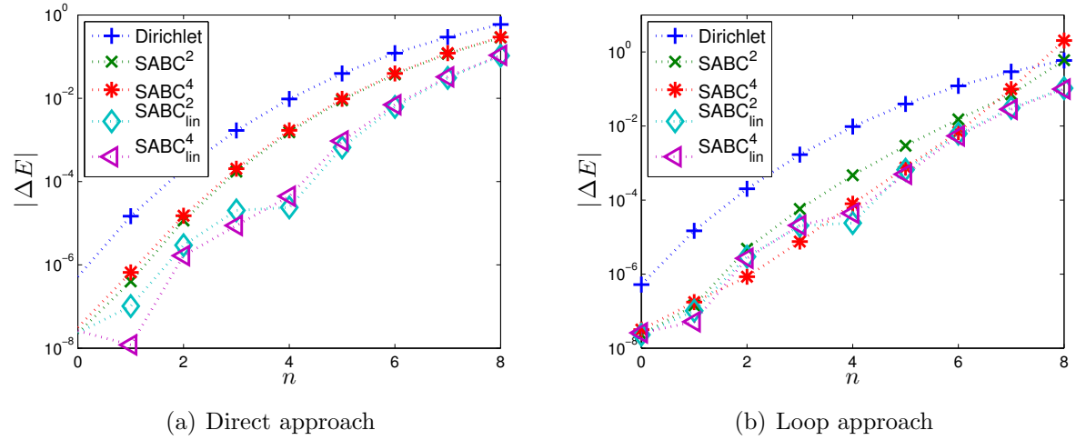
Figure 3: Example 1: Error on the eigenvalue depending on n ( \Omega = ]-4; 4[ ).
