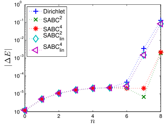
(b) x_r = 4 (loop)
