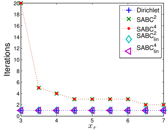
(b) n = 4
