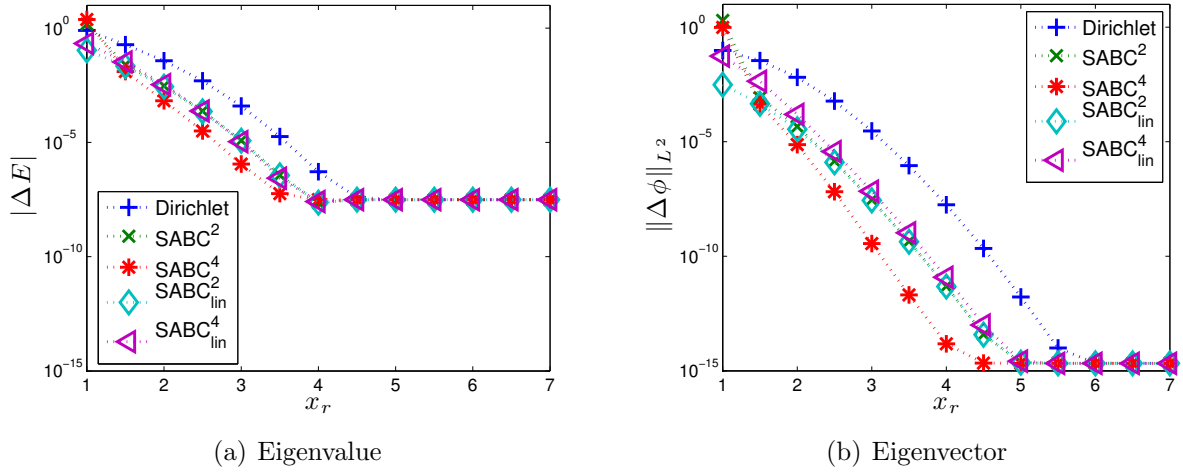
Figure 1: Example 1: Error ( n = 0 ).
